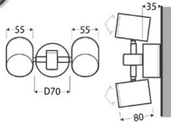
Double Spot Light surface mounted adjustable
