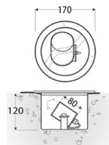
Lawn Light inground
