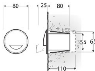
Step Light machined recessed
