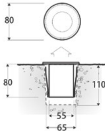
Up Light machined inground
