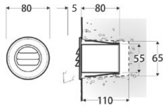
Step Light machined recessed
