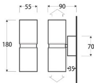
Up/Down Light surface mounted
