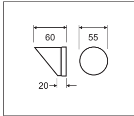
installation blockout (standard) MSBOS
