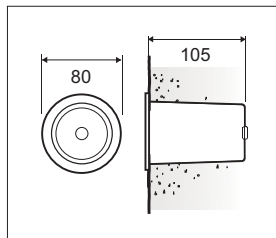
installation blockout (deep) MSBOD (deep)
